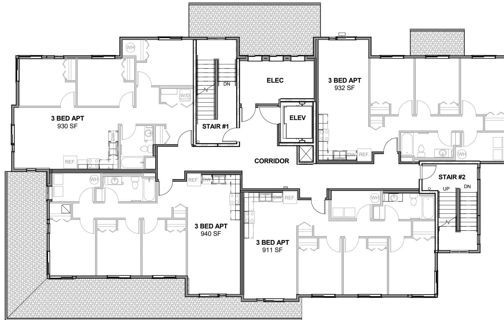
TYPICAL FLOOR PLAN AT BUILDING A
